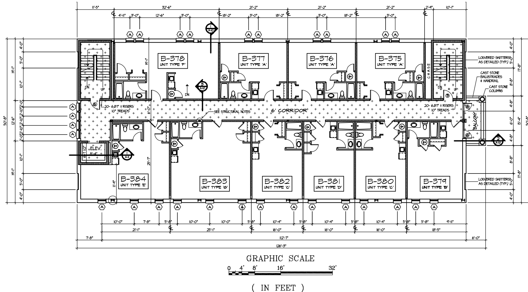
Building G: Arts Park Building, Third Floor Plan
