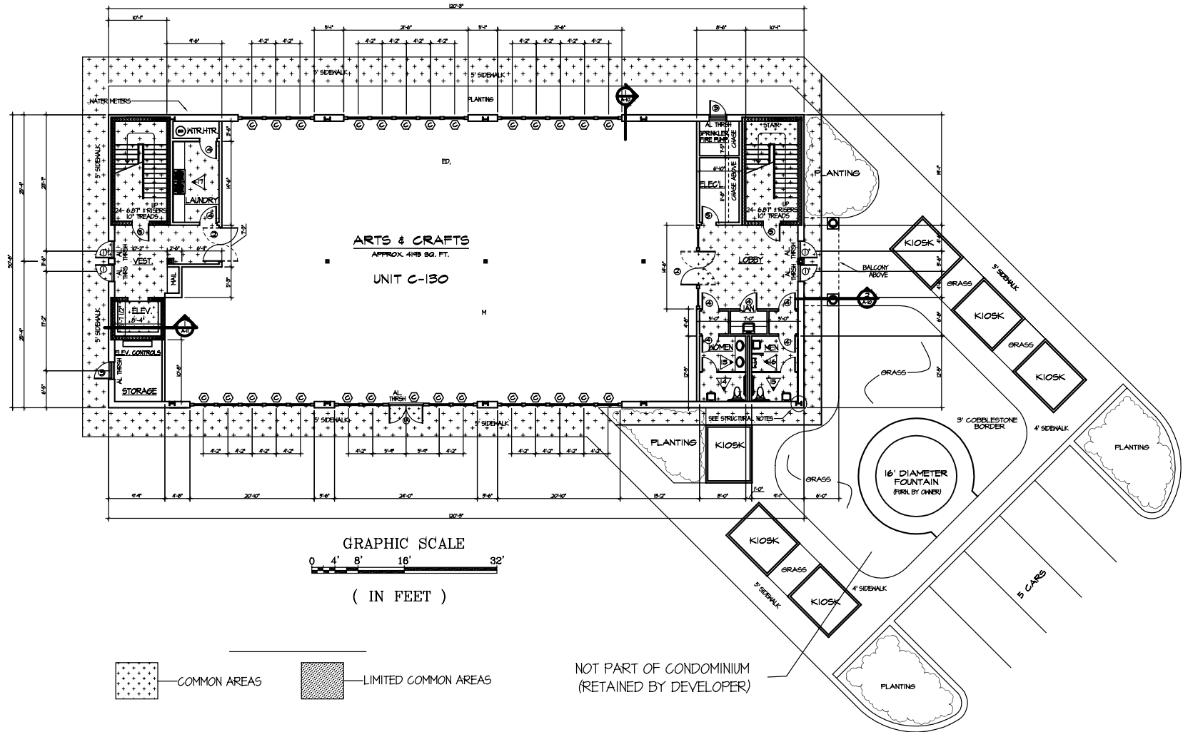
Building G: Arts Building, First Floor Plan
